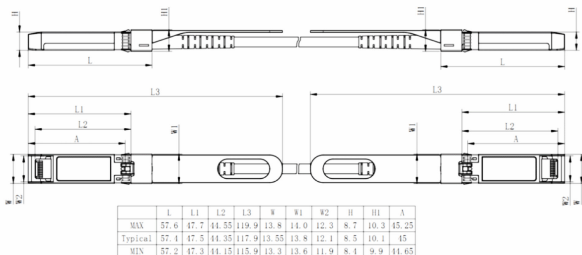
Figure 3. Mechanical Outline
