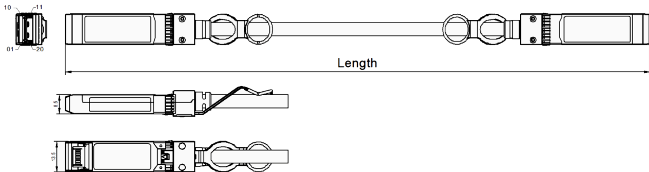
Figure 4. Mechanical Outline
